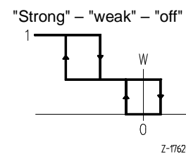
Fig. 4a Three-position control
