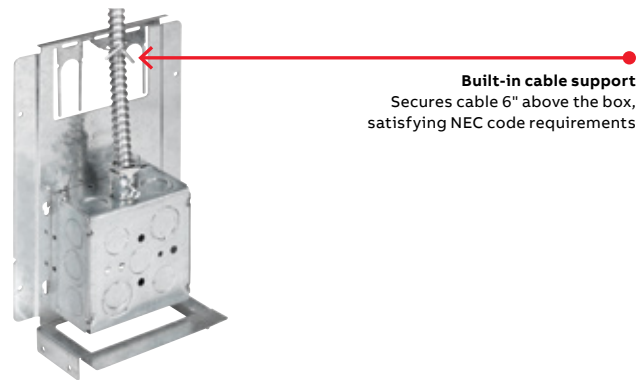
Back view of bracket with box, fitting and cable installed
