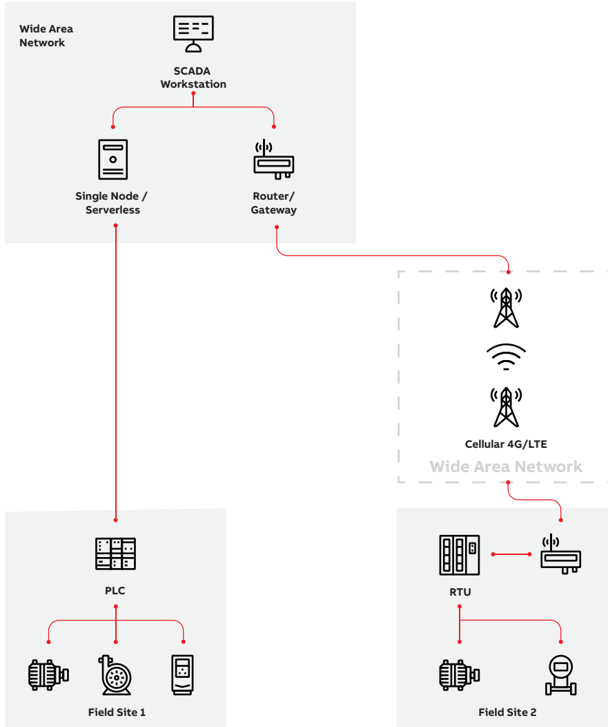
— 04 Single node or serverless architecture
