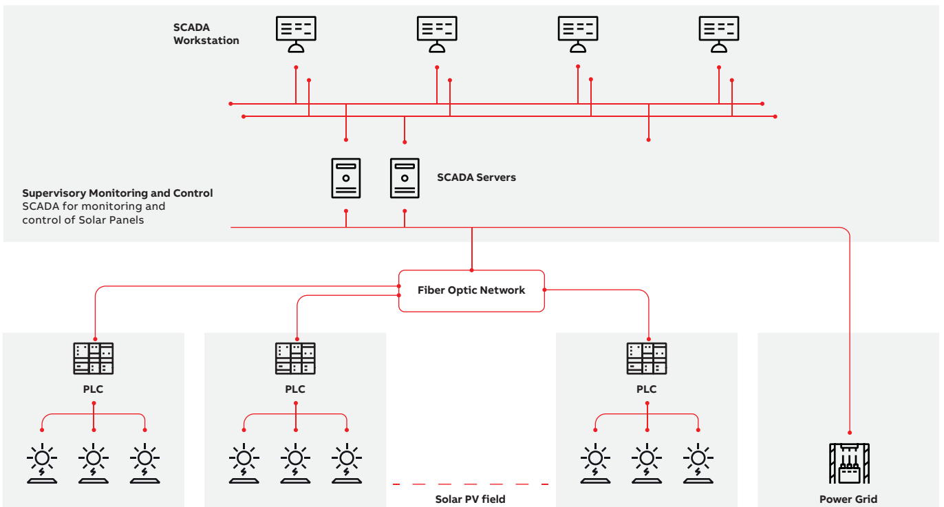
07 Supervisory monitoring of solar photovoltaic plants
