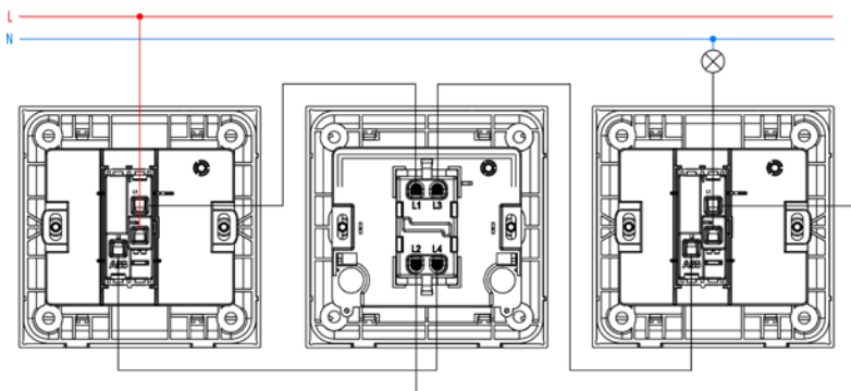
1G intermediate switch
