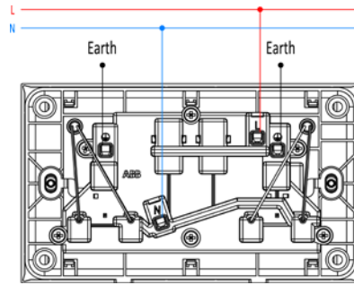
2G 13 A switch socket outlet SP
