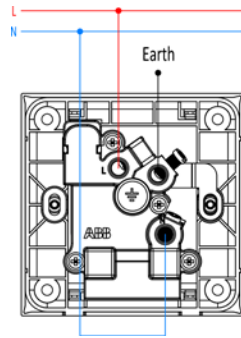
1G switch socket outlet
