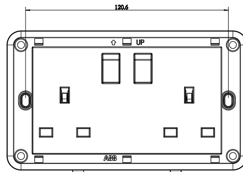
Distance between fixing screws for 2 gang frames
