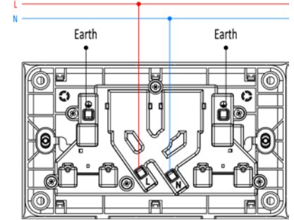
2G 13 A switch socket DP
