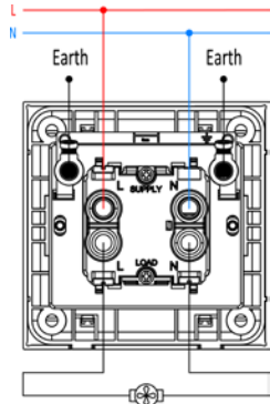
1G 1W 32 A (45 A) DP switch
