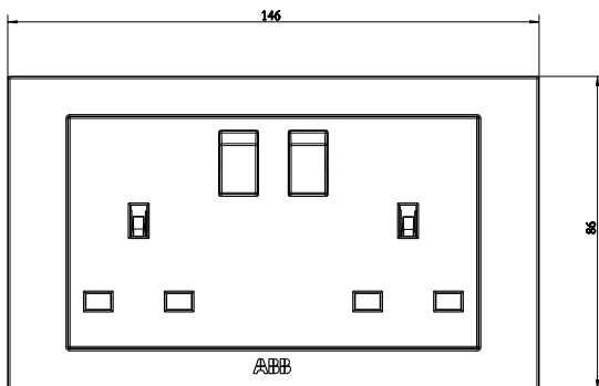
Dimensions for 2 gang frames
