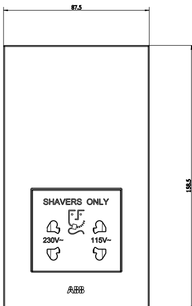
Dimensions for Shaver socket
