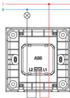
1G rotary dimmer
