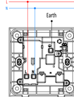
1G 13 A switch socket DP
