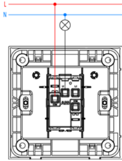
2G 1W switch
