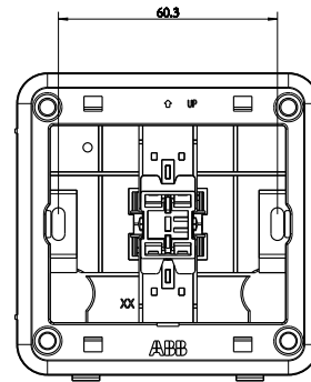
Distance between fixing screws for 1 gang frames
