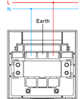
flex outlet 45 A
