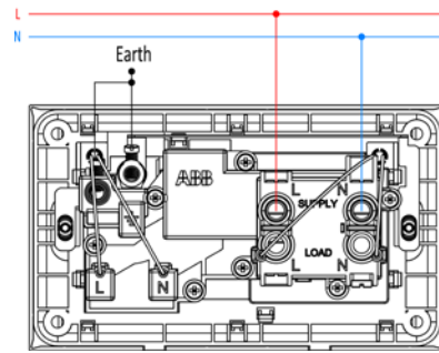
cooker control unit
