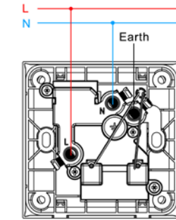
1G 15 A switch socket DP
