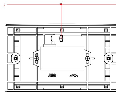
TV/FM splitter
