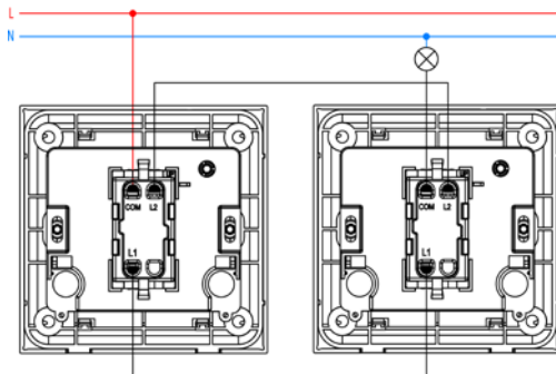
2G 2W 20 AX switch
