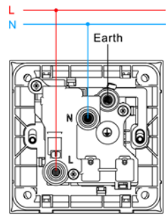
1G 5 A switch socket DP
