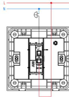
1G 1W push switch
