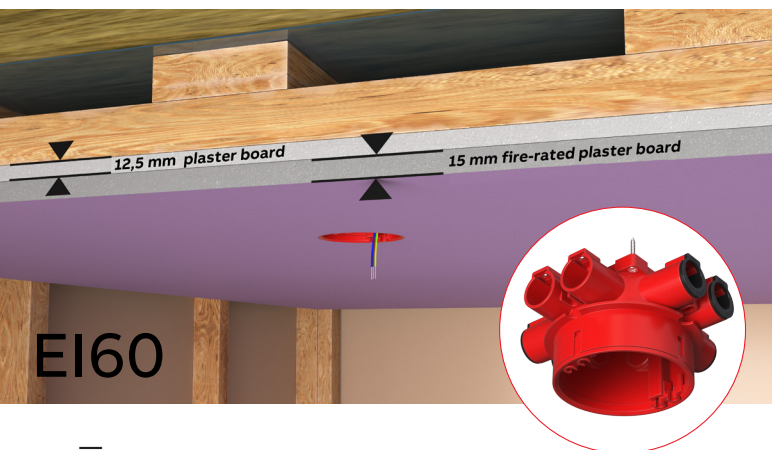
07 Installation on EI60 fire roof (1 x 12.5 mm plaster board and 1 x 15 mm fire plaster board). Red adapter ring raised in this position by 2.5 mm.
