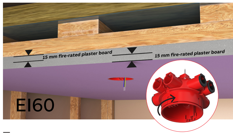
08 Installation on EI60 fire roof (2 x 15 mm fire plaster board). Red adapter ring raised in this position by 5 mm.
