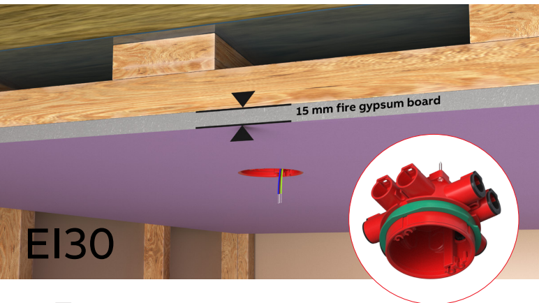
05 Installation on EI30 fire roof (1 x 15mm fire plaster board). A green elevation ring and a red adapter ring (raised in this position by 2.5 mm) are used.
