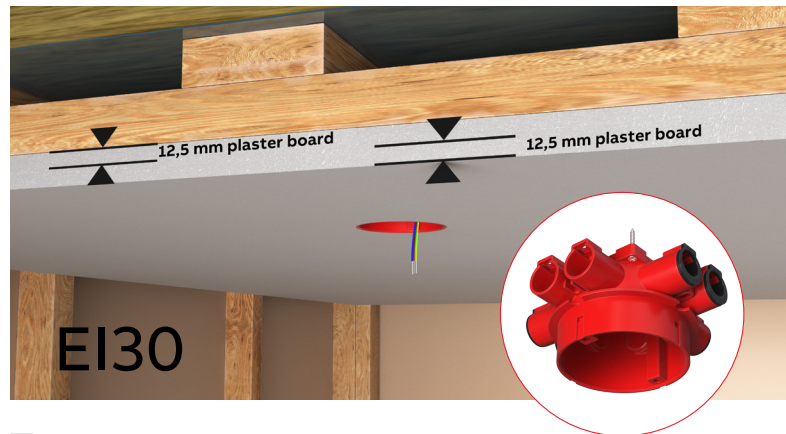
06 Installation on EI30 fire roof (with 2 x 12.5mm plaster board). No elevation or adapter rings.
