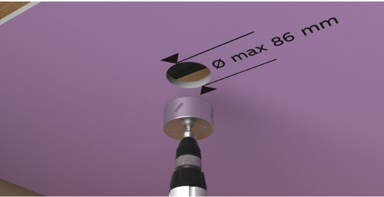
03 The mounting hole is made with a hole saw; the diameter of the hole must not exceed 86 mm.
