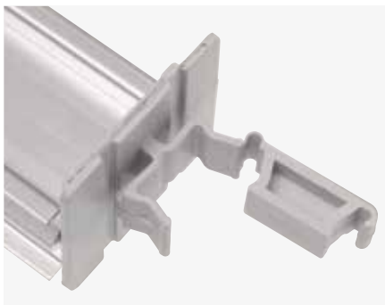
The DIN rail is supplied with special hooks already in position for attaching to the uprights.
