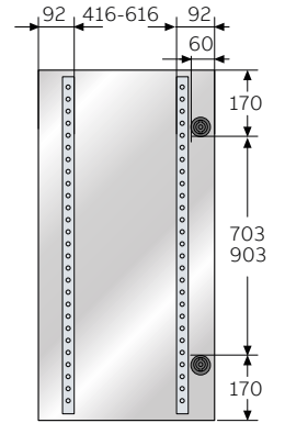
Doors H = 1000-1200
