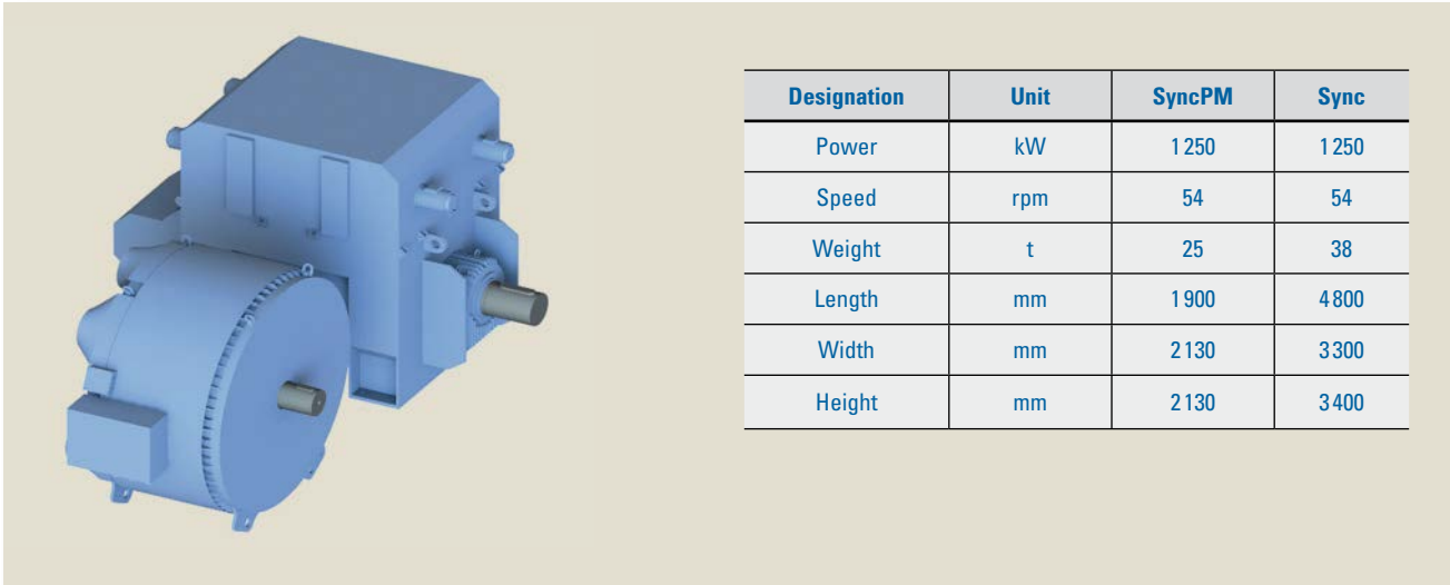
Figure 5: PM motor (left) vs. synchronous motor (right)
