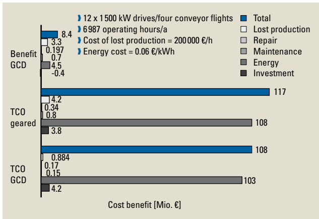
Figure 7: General example of cost benefit after having operated a gearless drive for over 15 years (TCO – Total Cost of Ownership)
