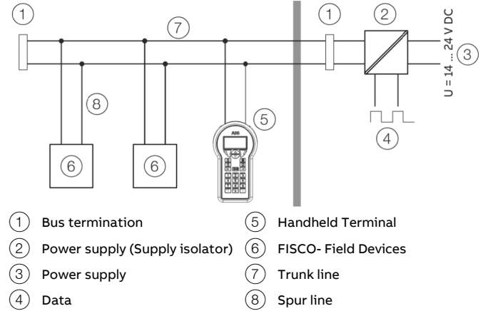
Figure 25: FISCO Control drawing (example)
