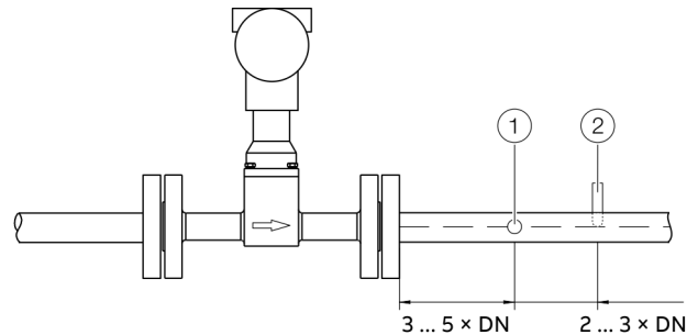
Figure 10: Arrangement of the temperature and pressure measuring points
