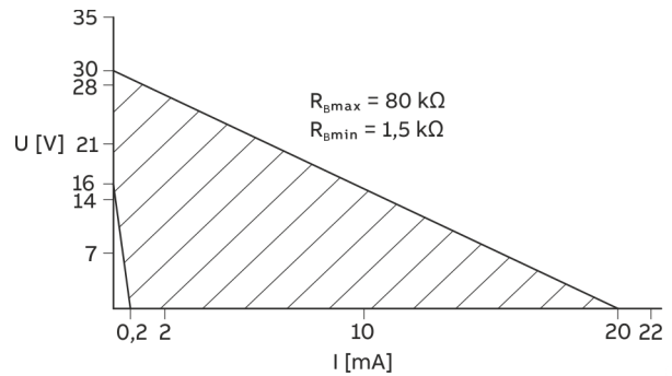
Figure 18: Range of the external supply voltage and current
