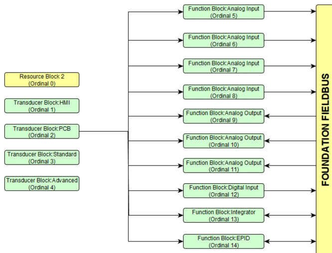
Figure 22: Design of the function blocks
