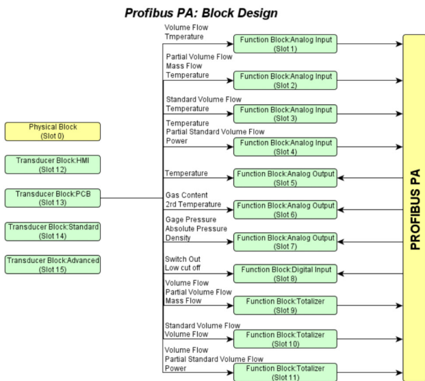
Figure 21: Design of the function blocks
