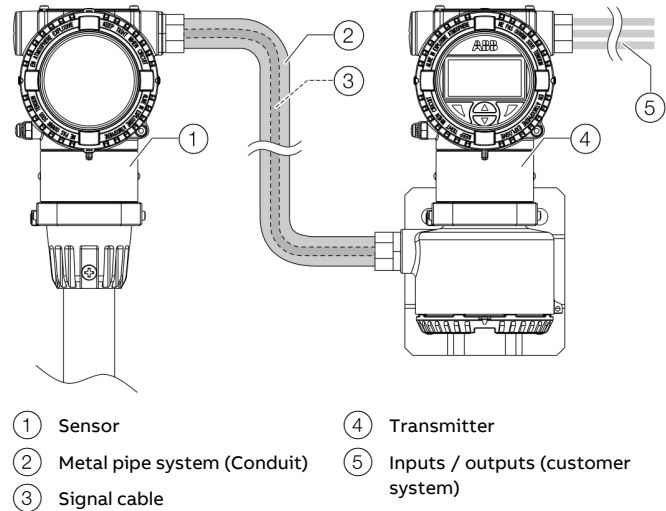
Figure 23: Signal cable installation with FM/CSA
