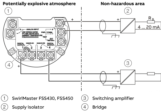
Figure 24: Electrical connection (example)
