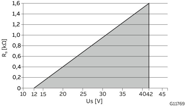
Figure 14: Load diagram of current output; load depending on supply voltage
