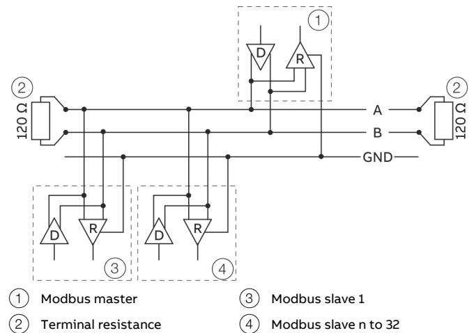
Figure 20: Modbus network (example)
