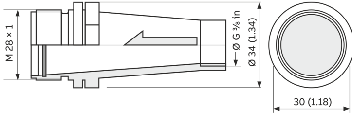
Screwed connection G 3/8 in, connection for Legris hose adapter, pair) for inlet and outlet; inlet adapter with high-tech flow conditioner
