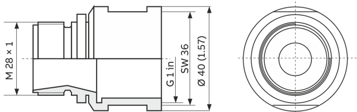
Screwed connection G 1 in
