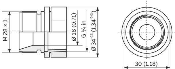
Screwed connection G 3/4 in, simultaneous connection for Transair system 25 mm (pair)
