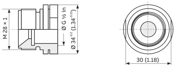
Screwed connection G 1/2 in (pair) for inlet and outlet; inlet adapter with high-tech flow conditioner
