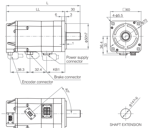
GYB motor (with brake)
