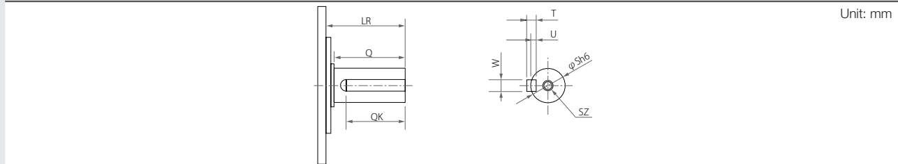
Shaft extension specifications [with key, tapped] Unit: mm
