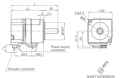
GYB motor (without brake)
