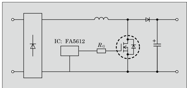
Fig.6 Circuit diagram of PFC demonstration board
