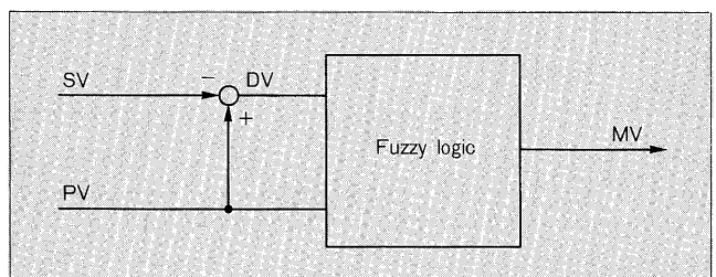
Fig. 5 Functional block diagram of PYX
