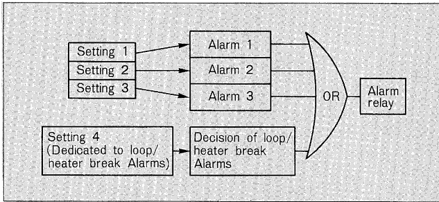
Fig. 9 Multi-alarm
