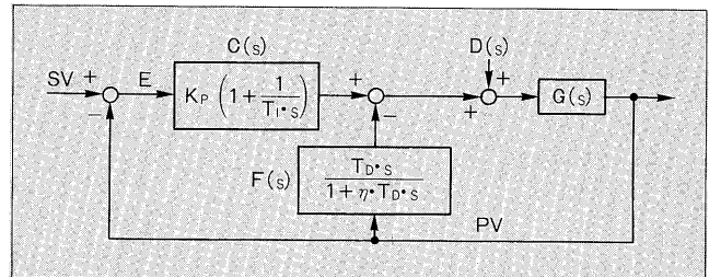
Fig. 3 One-degree of freedom PID
