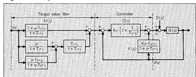
Fig. 4 Two-degrees of freedom PID (Target value filtering type)
