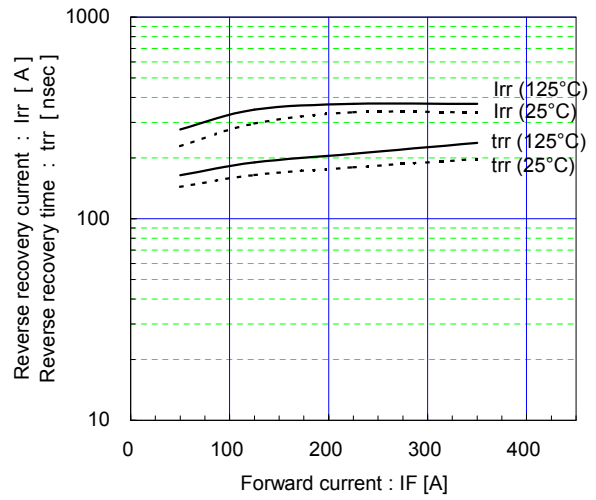
Reverse recovery characteristics (typ.) V_{cc}=900\text{V} , V_{GE}=\pm 15\text{V} , R_g=2.2\Omega
