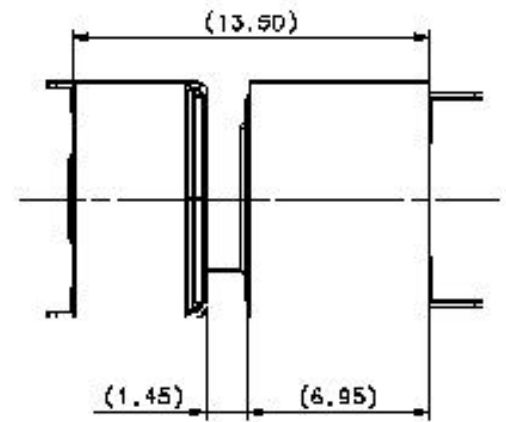
MATED CONDITION SCALE 4:1
