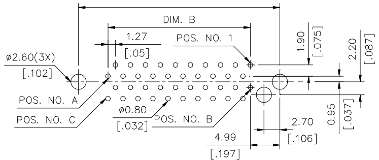
RECOMMENDED PC BOARD
