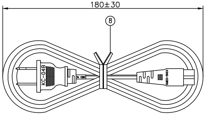
PACKING DRAWING
