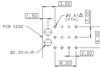
RECONNECTION PCB LAYOUT
