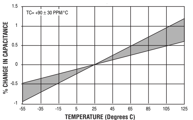
CAPACITANCE CHANGE VS. TEMPERATURE ATC SERIES 100, CASE C
